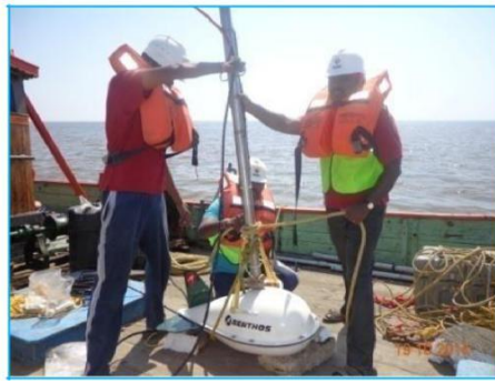
Shallow seismic survey
